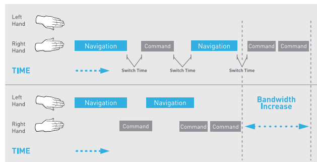
Fig. 1 - Comparison of single stream user input (one hand) vs. bi-manual (two handed) input stream. Notice how the user can "start" the command with the right hand while the left hand is completing the navigation.
