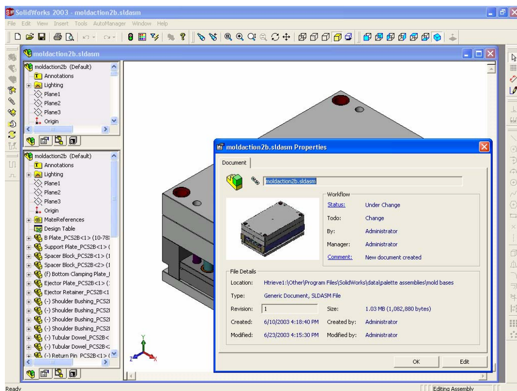
Figure 2 - AutoManager allows you to view and edit the document management properties directly from within SolidWorks
